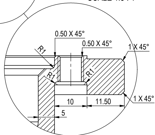
DETAIL F SCALE 1.5 : 1
